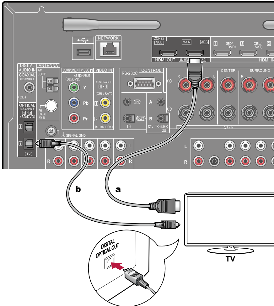
a HDMI cable, b Digital optical cable
