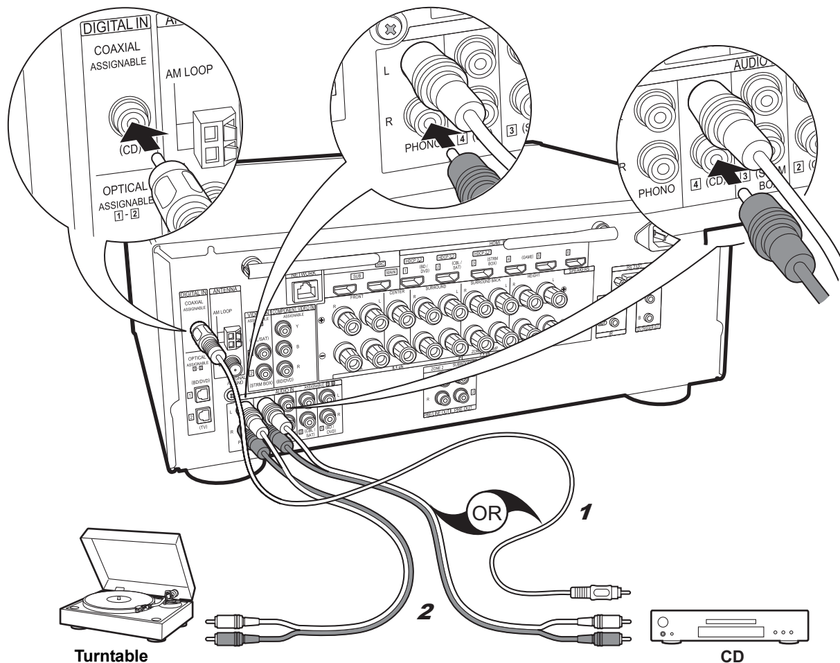
1 Digital coaxial cable, 2 Analog audio cable
