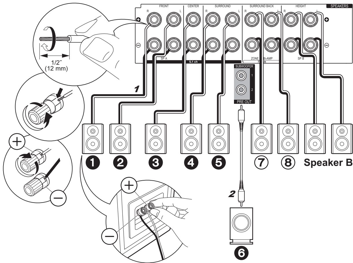
1 Speaker cable, 2 Subwoofer cable
