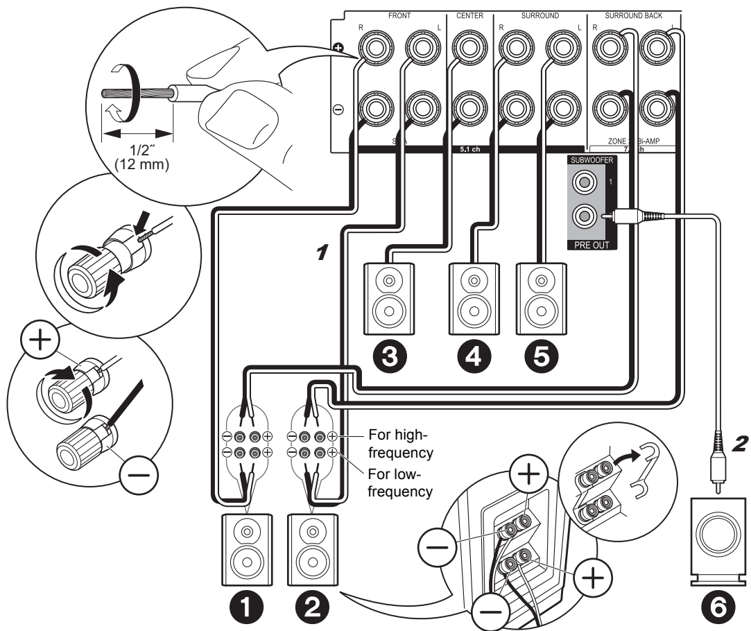
1 Speaker cable, 2 Subwoofer cable
