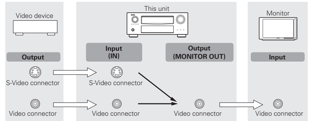
[Flow of video signals for ZONE2]
